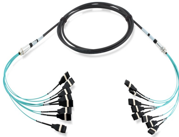
FO Trunk Cable with Dividing Element
