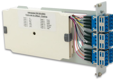
FO Compact Splice Module Twin 3U
